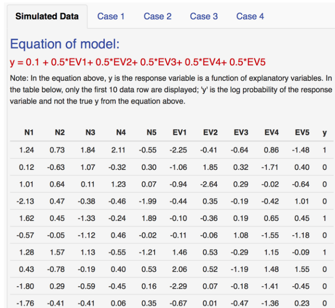
Fig. 7. Equation of the response variable and first 10 rows of the simulated dataset
